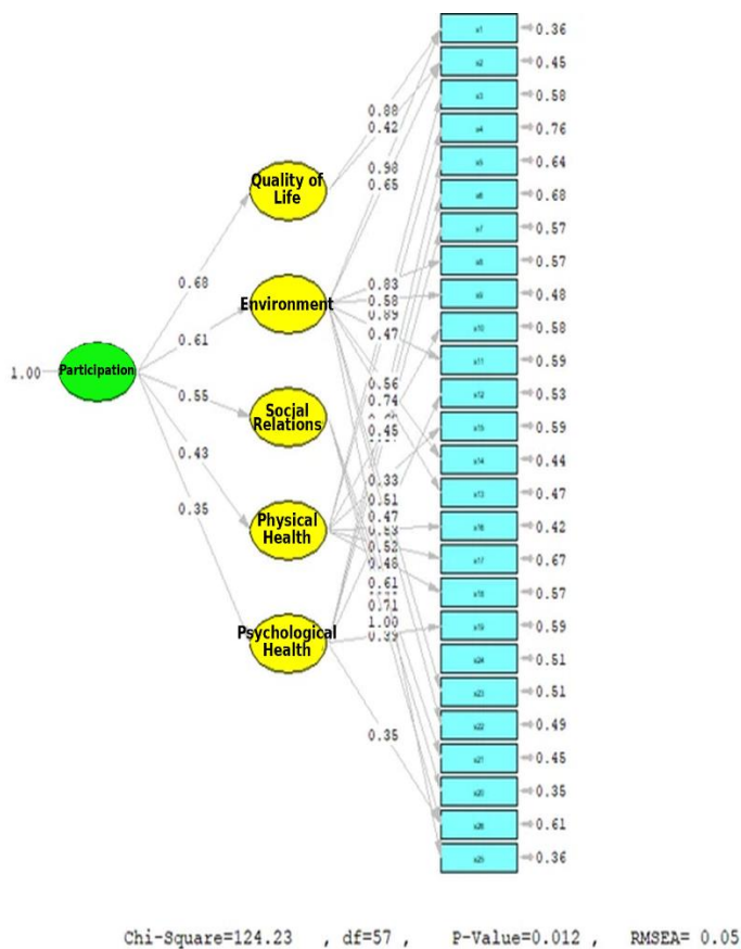
Figure 2. The research structural model showing standardized coefficient estimates, item factor loadings, and measurement error variances.
